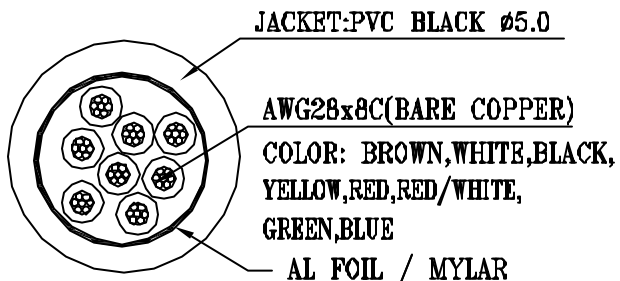
WIRE 1# CONFIG DETAIL
